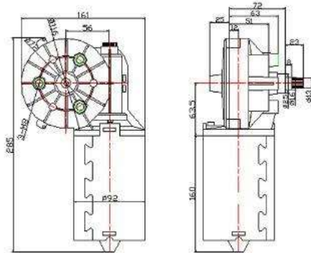
150W,24V/12V
